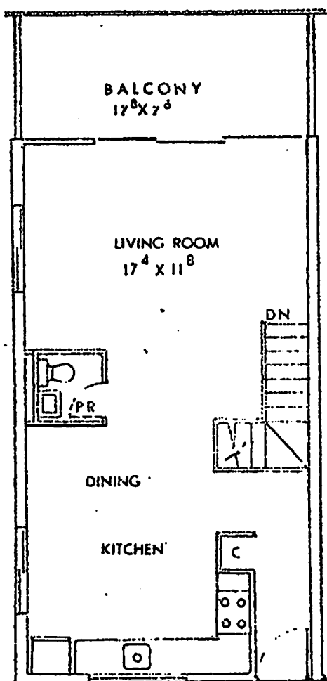
UPPER FLOOR
